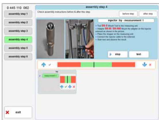
Air Gap Testing Screen
