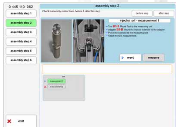
Test Screen of CARS Control Software
